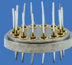
Hermetic Feedthrough Hermetic feedthroughs using ceramic-to-metal seals.
